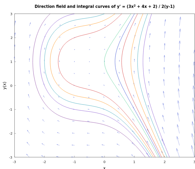
Figure 5.8: The direction field and integral curves of \frac{dy}{dx} = \frac{3x^2+4x+2}{2(y-1)} (Hamzstplot/Examples with Makefile/Plot First Order Differential Equation Direction Field and Solutions Curves for Separable Equations Example 2/main.cpp).
