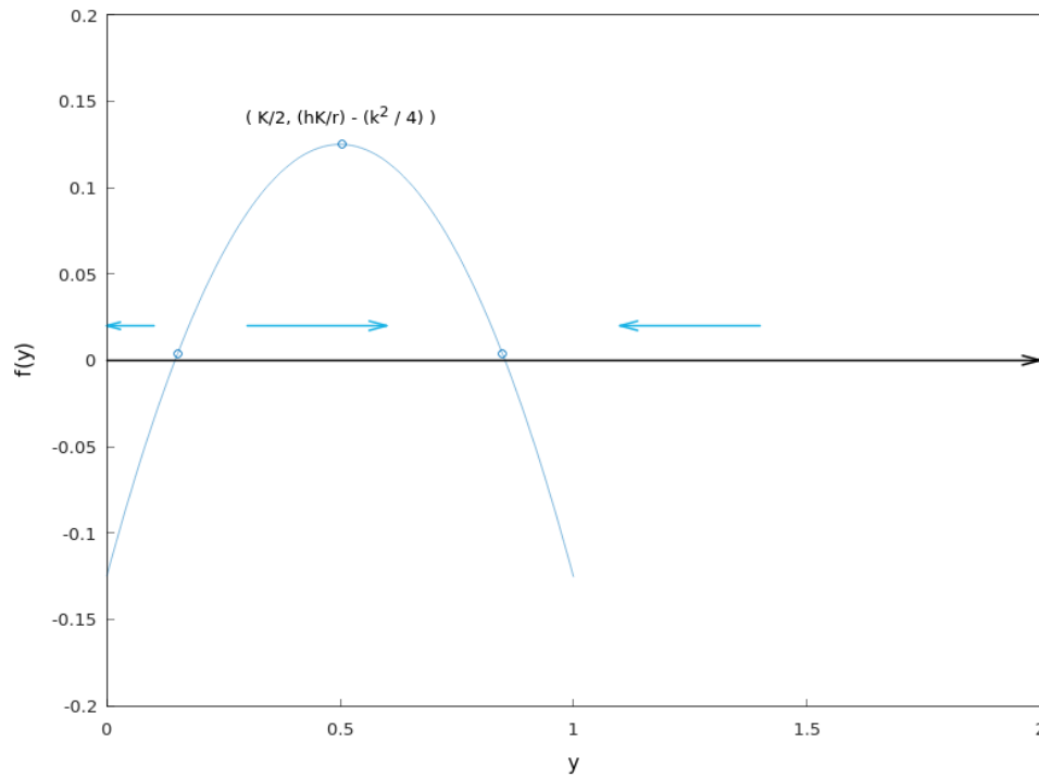
Figure 5.18: The plot for f(y) = (1 - y)y - \frac{1}{8} (Hamzstplot/Examples with Makefile/Plot 2D Equilibrium Solution for Schaefer Model Variation/main.cpp).
