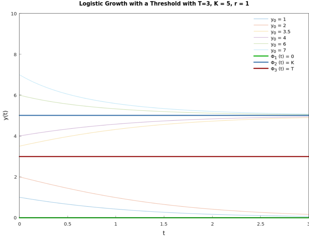
Figure 5.15: The solution curves for logistic growth with a threshold for \frac{dy}{dt} = -r \left(1 - \frac{y}{T}\right) \left(1 - \frac{y}{K}\right) y (Hamzstplot/Examples with Makefile/Plot 2D Solution Curves for Logistic Growth with a Threshold/main.cpp).
