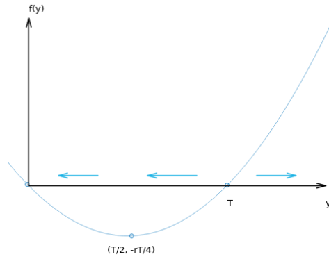
Figure 5.12: The graph of f(y) for \frac{dy}{dt} = -r \left(1 - \frac{y}{T}\right) y (Hamzstplot/Examples with Makefile/Plot 2D Equilibrium Solution for Critical Threshold/main.cpp).
