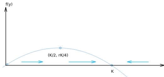
Figure 5.9: The equilibrium solution f(y) = 0 or r(1 - y/K)y = 0 to visualize other solutions of Eq. (4.53) ( Hamzstplot/Examples with Makefile/Plot 2D Equilibrium Solution for Logistic Growth/main.cpp ).
