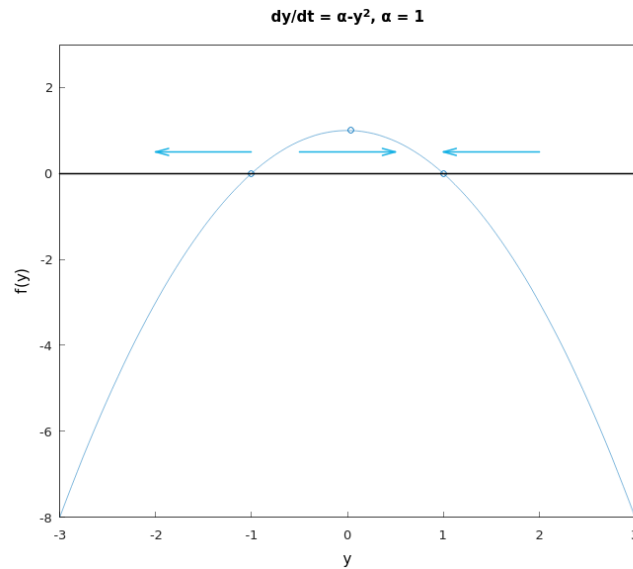
Figure 5.24: The plot for f(y) = \alpha - y^2 with \alpha = 1 , the phase line is drawn with the blue arrows ( Hamzstplot/Examples with Makefile/Plot 2D for Bifurcation Points Problem 25 2 Equilibrium Solutions/main.cpp ).
