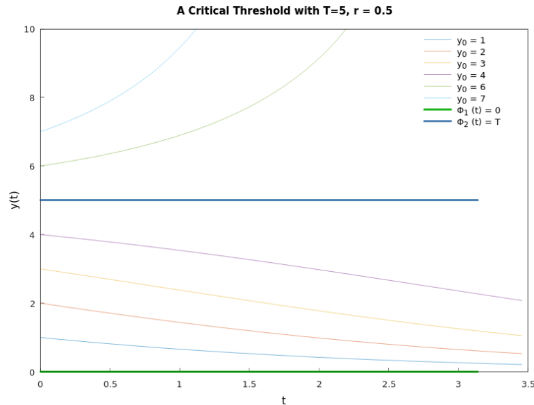
Figure 5.13: The solution curves for growth with a threshold for \frac{dy}{dt} = -r \left(1 - \frac{y}{T}\right) y (Hamzstplot/Examples with Makefile/Plot 2D Solution Curves for Critical Threshold/main.cpp).
